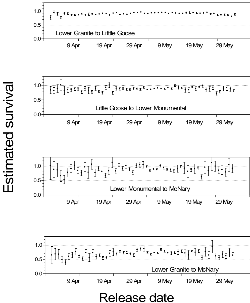
Figure 2. Estimated survival through various reaches vs. release date at Lower Granite Dam for daily release groups of Snake River yearling Chinook salmon, 2005. Bars extend one standard error above and below point estimates.
